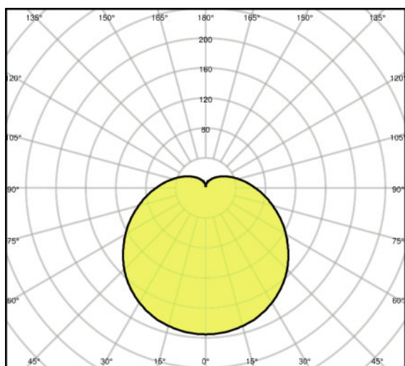
cd/klm = 100% — C0/C180 — C90/C270
