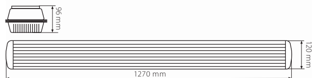
● DICT-236/PC/PS
