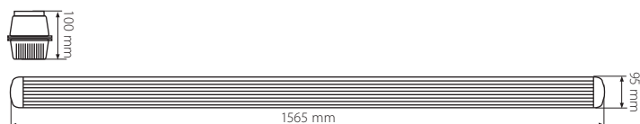
● DICT-158/PC/PS
