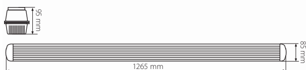
● DICT-136/PC/PS
