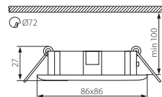
FIRLA CT-DTL50
