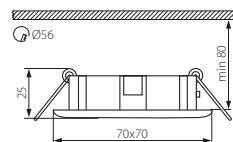
FIRLA CT-DTL35
